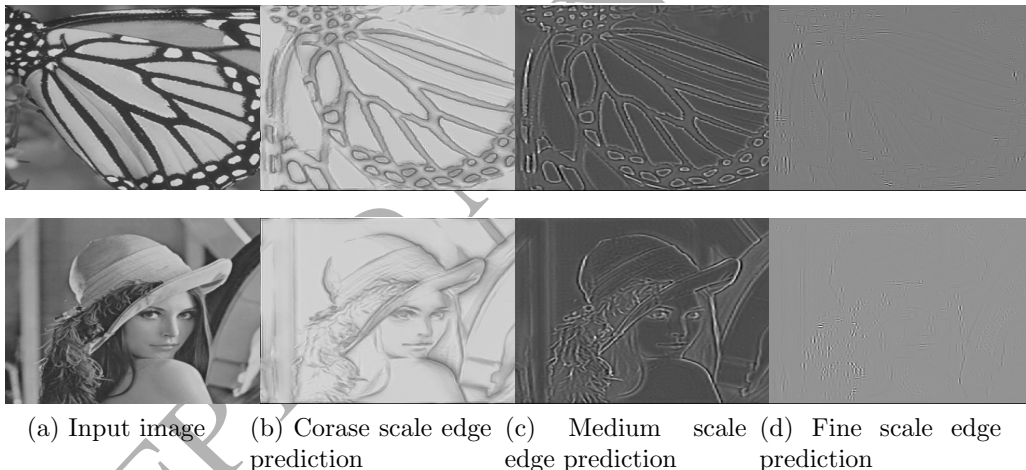
Figure 8: Multi-scale edge prediction extracted from a network training session. From left to right: original image, coarse scale (4 layers) edge prediction, medium scale (8 layers) edge prediction and fine scale (12 layers) one.
