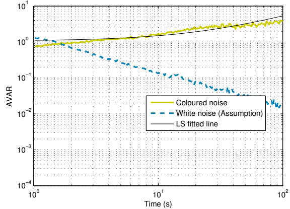
Fig. 6. AVAR and the LS fitted line of the NLOS scenario with a human block.
