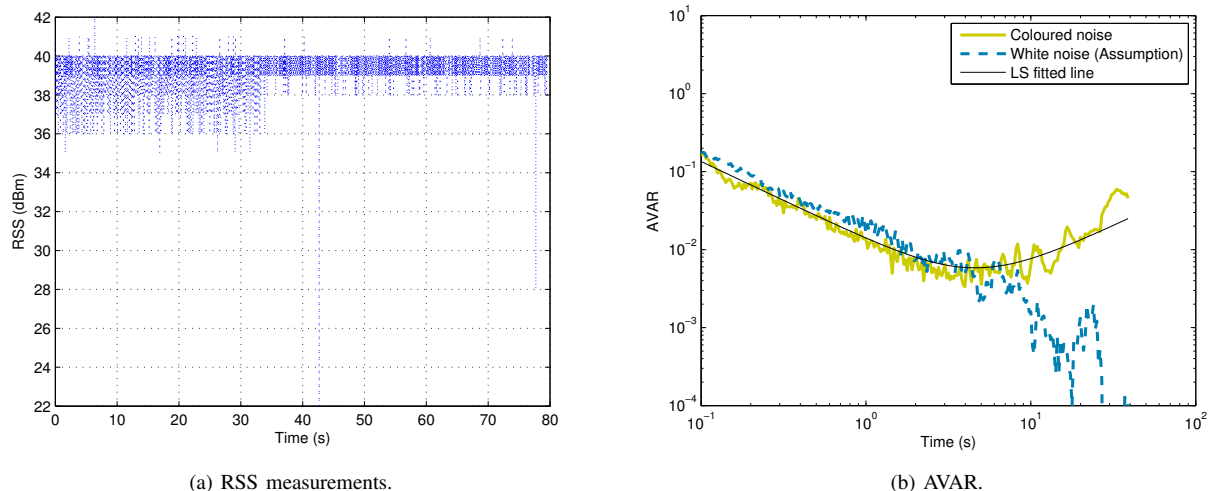
Fig. 9. The RSS measurements and AVAR (90 degree).
