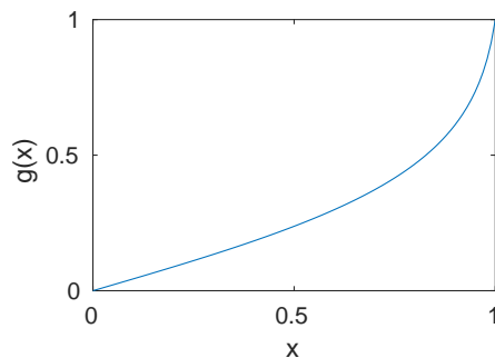
Figure 3. Plot of a non-linear function g(x) where g(0) = 0 and g(1) = 1 .
