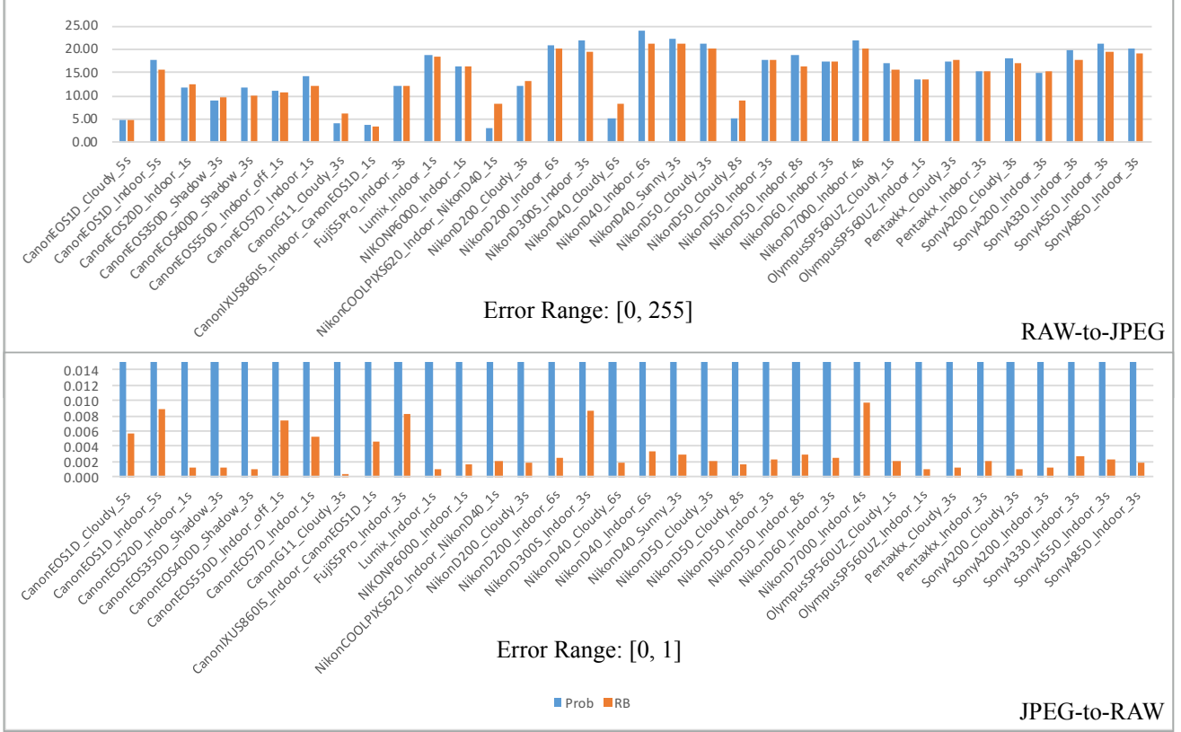
Figure 5. Test RMSE bar chart of the NUS dataset [18] for Prob [5] and our RB [17]. The figure shows RMSE between ground truth and prediction for bidirectional raw and JPEG mappings. The horizontal and vertical axes indicate camera sensor model code and calibration error respectively. The displayed forward and backward errors are clipped at 25.0 and 0.015 respectively. The displayed errors are the mean errors of all capture conditions.
