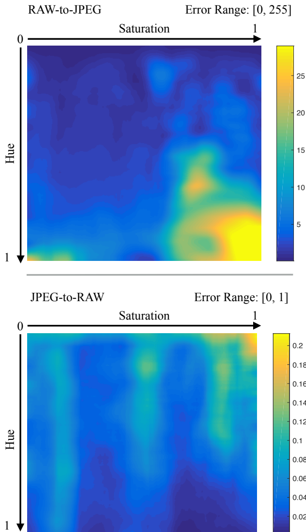
Figure 6. Distributions of forward and backward mapping RMSE of our method over the input hue and saturation gamut. It is tested with the “1 illuminant + 10 exposures” set from the Harvard dataset [5].
