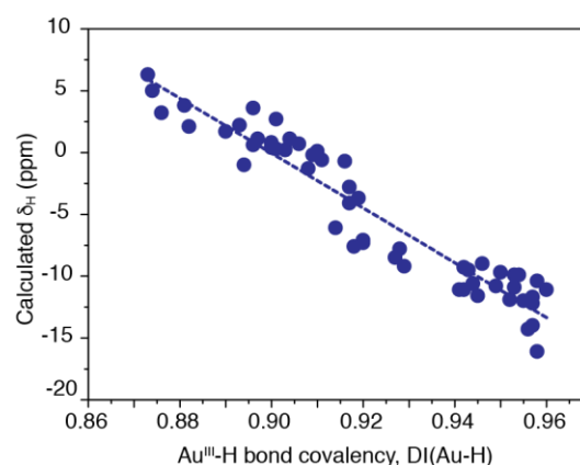
Figure 6. Correlation of computed ^1\text{H} NMR hydride shifts (in ppm vs. TMS) with QTAIM delocalization indices, DI(Au-H), as a measure of the bond covalency, for a series of mononuclear Au(III) hydride complexes (cf. SI, Tables S2-S4 for numerical data).
