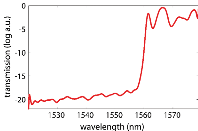
FIGURE 7 Example of transmission spectrum for one of the biofunctionalized photonic bandgap (PBG) sensing structures
