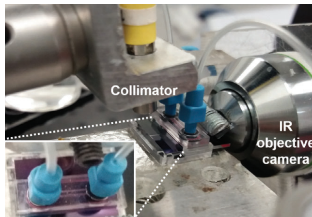
FIGURE 6 Picture of the assembled photonic sensing chip placed on the interrogation platform and detailed image of the flow cell having the microfluidic channel on its bottom side
