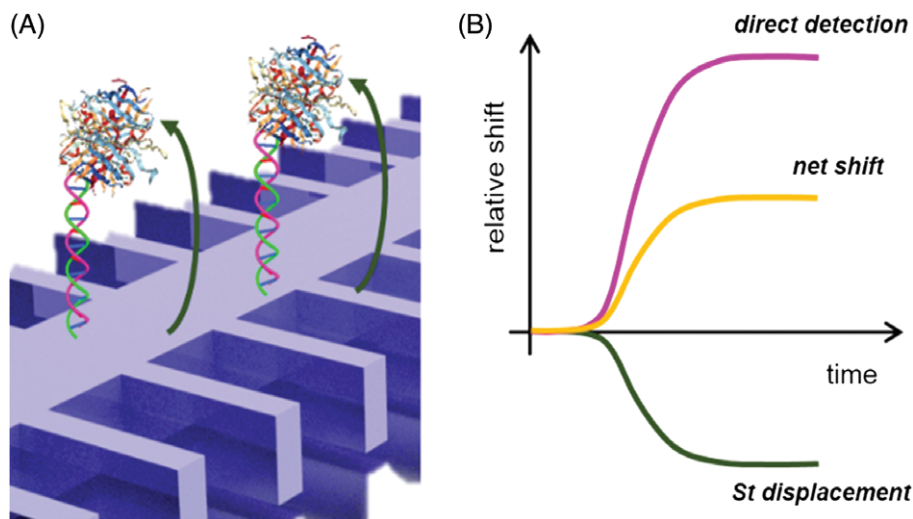
FIGURE 10 A, Schematic representation of the displacement of the streptavidin from the surface of the photonic bandgap (PBG) sensing structure when the molecular beacon (MB) changes its conformation due to the hybridization with the target oligonucleotide. B, Schematic representation of the photonic sensor response when streptavidin-labeled MB probes are used. The final net response is a result of the combination of the positive shift given by the direct recognition of the target oligonucleotide and of the negative shift given by the streptavidin displacement
