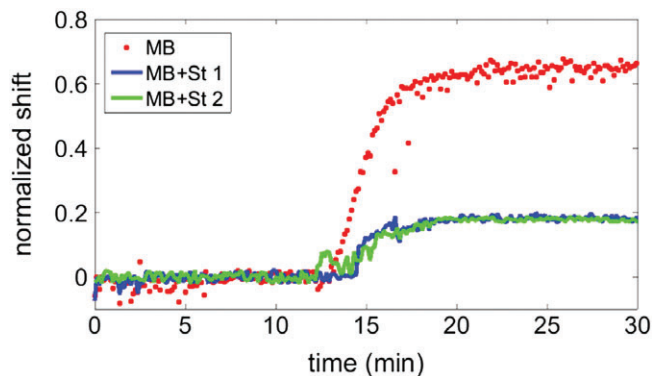
FIGURE 9 Normalized temporal evolution of the photonic bandgap (PBG) edge position of the sensing structures. The normalized sensing response for the PBG structure being biofunctionalized with the streptavidin-free molecular beacon (MB) probes is depicted with red dots, while the sensing response of the PBG sensing structures being biofunctionalized with the streptavidin-labeled MB probes are depicted with green and blue solid lines
