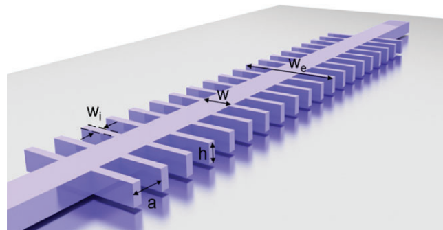
FIGURE 4 Schematic representation of the selected photonic bandgap (PBG) sensing structure. The periodic silicon photonic structure is placed on top of a silicon oxide lower cladding. Note that the linear access taper is not included in the scheme
