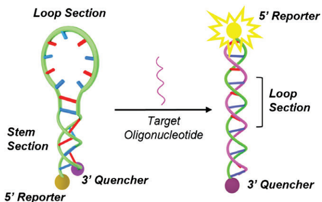
FIGURE 1 Schematic explanation of the working principle of a fluorescence-based molecular beacon (MB) probe for oligonucleotide detection
