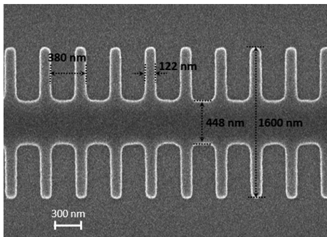
FIGURE 5 Scanning electron microscope (SEM) image of a fabricated photonic bandgap (PBG) sensing structure
