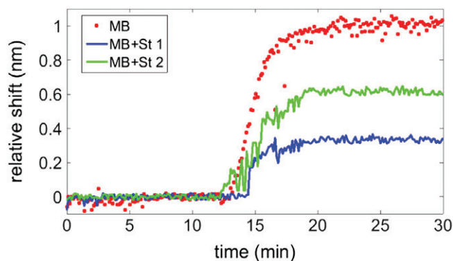
FIGURE 8 Temporal evolution of the photonic bandgap (PBG) edge position of the sensing structures when the target oligonucleotide strand is flown over the sensors. The sensing response for the PBG structure being biofunctionalized with the streptavidin-free molecular beacon (MB) probes is depicted with red dots, while the sensing response of the PBG sensing structures being identically biofunctionalized with the streptavidin-labeled MB probes (MB + St 1 and MB + St 2) are depicted with green and blue solid lines
