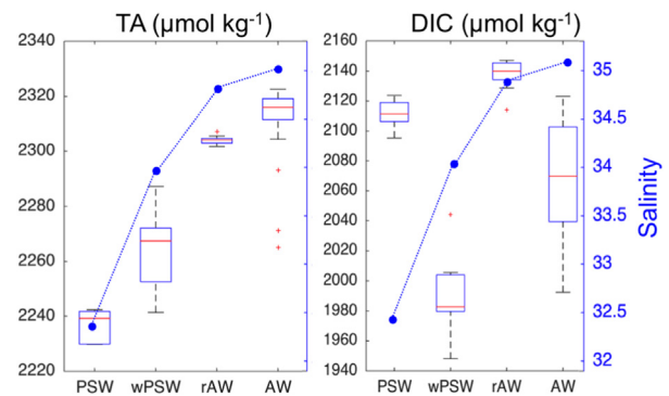
Fig. 9. Average salinity, total alkalinity (TA) and dissolved inorganic carbon (DIC) concentrations for water masses in the Fram Strait (PSW: Polar Surface water; wPSW: warm Polar Surface Water; AW: Atlantic Water; rAW: recirculated Atlantic Water); The red line is the median, the edges of the box are the 25th and 75th percentiles, and the whiskers show the range of values not considered outliers. (For interpretation of the references to colour in this figure legend, the reader is referred to the web version of this article.)
