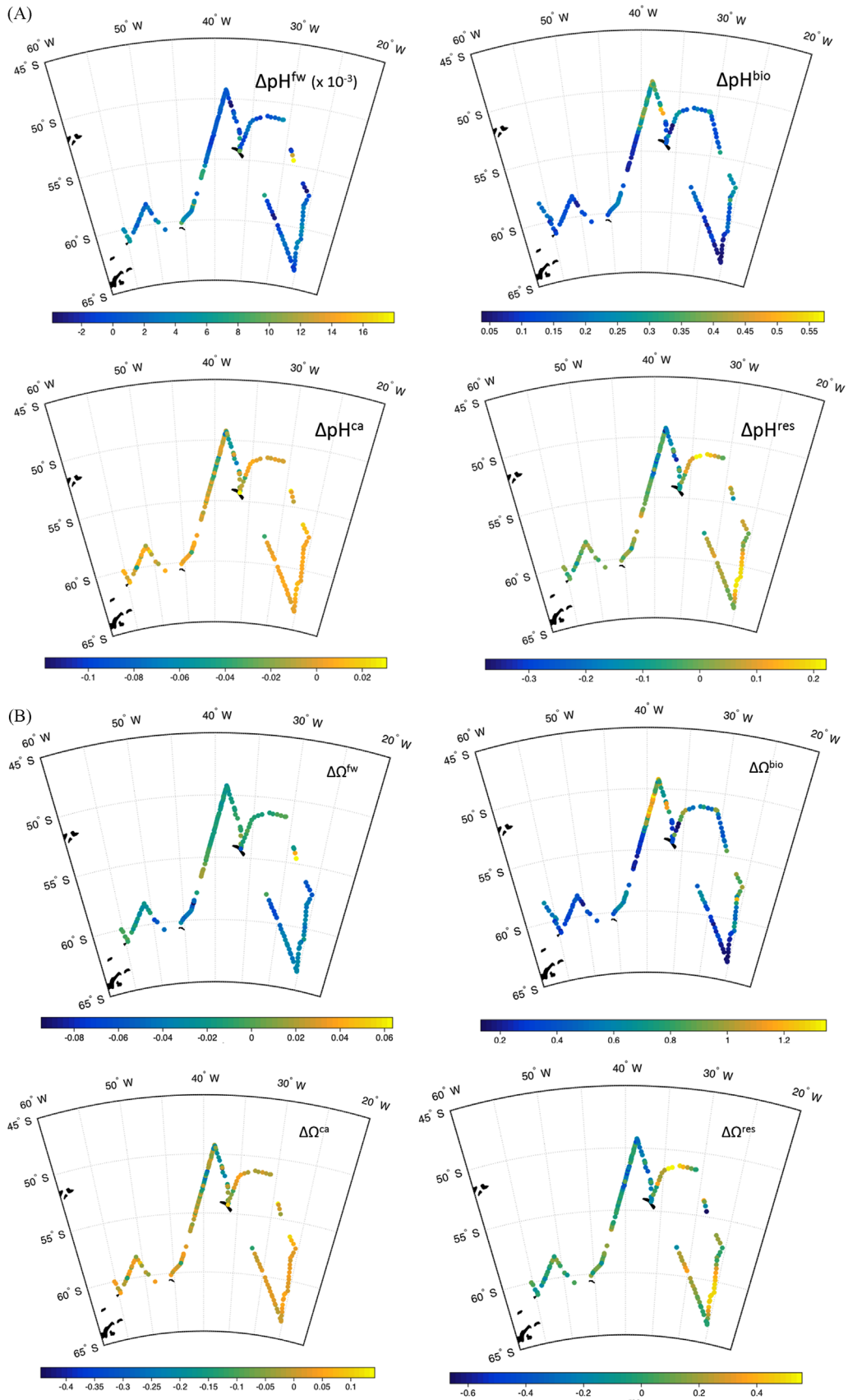
Fig. 7. Components of the net seasonal changes in (a) pH and (b) \Omega_{ar} as determined by analysis of the WW layer (Sections 3.4 and 5.1). Components are fw=freshwater, bio=biological, ca=calcification, and resid=residual (i.e. physical processes), as discussed in the text.
