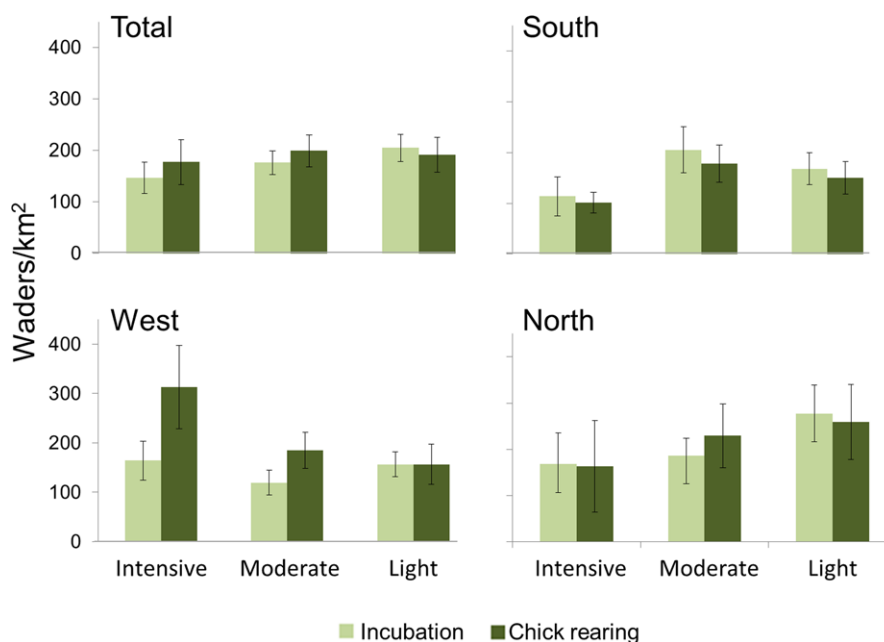
Figure 3 Mean ( \pm SE ) densities of the seven most common wader species on the three different management types in the early (light green) and late (dark green) season surveys across all survey sites (total) and in each of the three regions (see Fig. 1 for regions).
