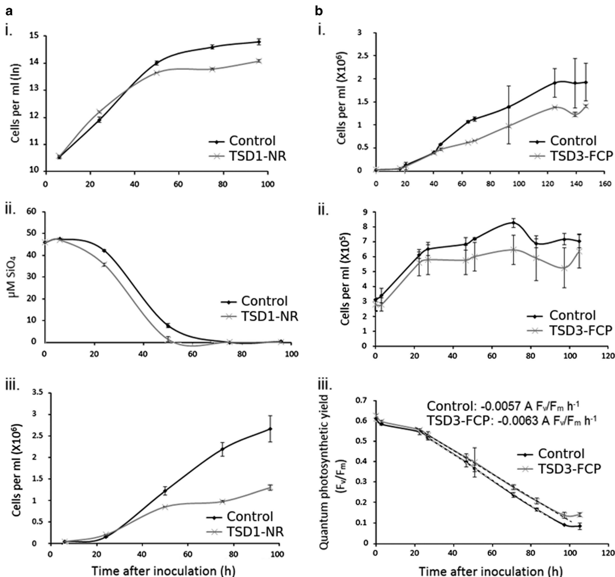
Figure 2 (a) Growth of TSD1-NR cells compared with a NAT control cells in silica-starved medium. i: natural log of cell abundance per ml; ii: \text{Si(OH)}_4 content of the medium; iii: cell abundance per ml. (b) Growth of NAT and TSD3-FCP cells under nitrogen starvation i: cell abundance per ml in nitrate-starved medium (containing 0.1 mM \text{NaNO}_3 at the beginning of the experiment); ii: cell abundance per ml after transfer from replete to nitrogen-free medium; iii: quantum photosynthetic yield ( F_v/F_m ) of cultures after transfer from replete to nitrogen-free medium. The slope of change in quantum photosynthetic yield over time is given and highlighted by dashed lines. Error bars represent s.d. of biological triplicate samples in all graphs.
