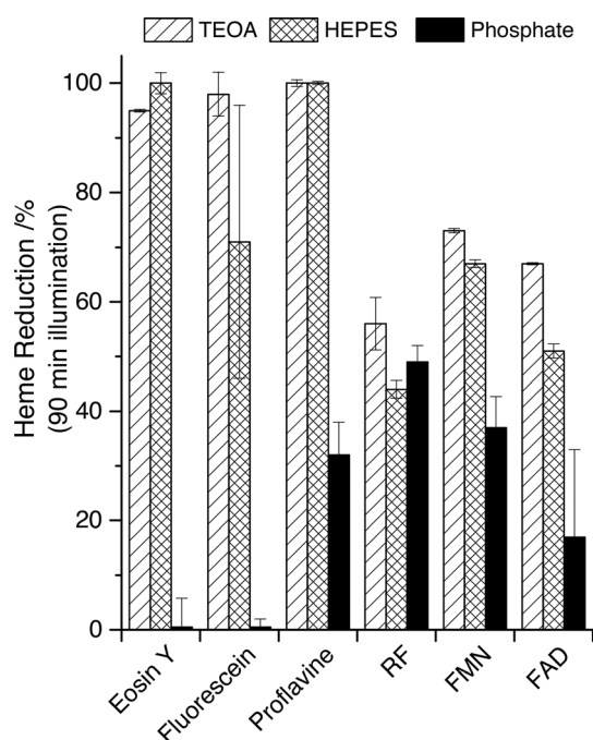
Figure 5. Impact of SED on the extent of OmcA photoreduction triggered by 90 min illumination. Extent of heme reduction (%) after 90 min illumination ( \lambda > 390 \text{ nm} , power \approx 400 \text{ W m}^{-2} ) of 0.5 \mu\text{M} OmcA at pH 7, 20^\circ\text{C} with 10 \mu\text{M} of each indicated photosensitizer in anaerobic 50 mM phosphate (inactive as SED) or with 50 mM TEOA, or 50 mM HEPES, as indicated. Heme reduction was quantified by change in electronic absorbance at 552 nm except in the case of eosin Y, in which spectral overlap of contributions from the photosensitizer and protein at this wavelength necessitated an equivalent analysis for the Soret peak at 420 nm (see text for details). Extents of reduction are the averages of two experiments and the errors are the differences between the average and the maximum and minimum values.
