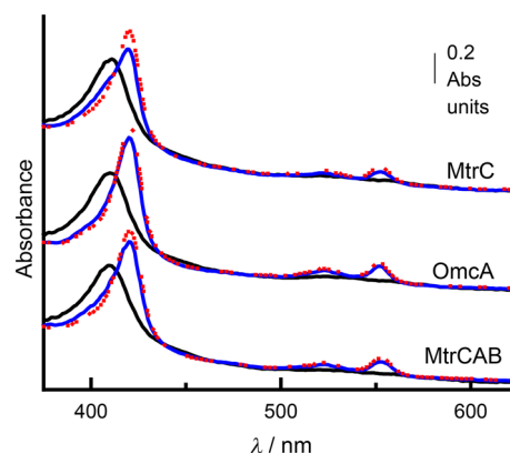
Figure 7. Photoreduction of MtrC, OmcA, and MtrCAB solutions by RuP- \text{TiO}_2\text{-MtrC} particles. Electronic absorbance of RuP- \text{TiO}_2\text{-MtrC} suspensions (0.037 \text{mg mL}^{-1} ) with 0.65 \mu\text{M} MtrC (top), 0.61 \mu\text{M} OmcA (middle), and 0.31 \mu\text{M} MtrCAB (bottom) before (black) and after (blue) 30 min illumination ( \lambda > 390 nm, power \approx 400 \text{W m}^{-2} ), followed by the addition of excess sodium dithionite (red). Experiments performed at 20 °C in anaerobic 150 mM MES (pH 6) with Triton X-100 (0.2%, v/v) included for MtrCAB. Spectra offset on the y-axis for clarity.
