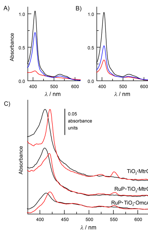
Figure 6. Adsorption and photoreduction of MtrC and OmcA on (RuP-)TiO 2 particles. Electronic absorbance of A) MtrC and B) OmcA solutions (1 \mu M, 200 \mu L) before (black) 30 min incubation with TiO 2 particles (0.5 mg mL -1 ) in 150 mM MES (pH 6) followed by centrifugation to pellet the particles and retrieval of the supernatant (red). The protein-coated particles were resuspended in 200 \mu L of 25 mM phosphate, 150 mM MES (pH 6) and incubated for 30 min to release the bound protein. The particles were pelleted by centrifugation, and spectroscopy of the supernatant (blue) quantified the released protein. C) Electronic absorbance recorded with an integrating-sphere spectrophotometer for suspensions (0.055 mg mL -1 ) of (RuP-)TiO 2 -MtrC (OmcA) particles as indicated. Spectra are presented after subtraction of the response from unmodified particles and offset on the y-axis for clarity; TiO 2 -MtrC particles before (black) and after (red) addition of excess sodium dithionite (top), RuP-TiO 2 -MtrC particles before (black) and after (red) 20 min illumination (middle), RuP-TiO 2 -OmcA particles before (black) and after (red) 10 min illumination (bottom). Experiments performed in anaerobic 150 mM MES (pH 6), 20 °C. Illumination \lambda > 390 nm, power \approx 400 W m -2 .
