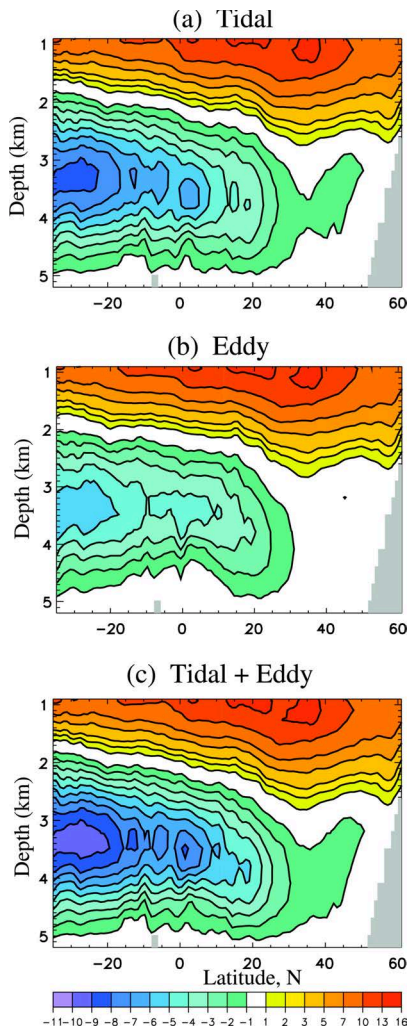
Fig. 7. Mean overturning circulation (Sv) below about 1 km depth in (a) tidal, (b) eddy, and (c) tidal+eddy experiments. Negative values correspond to counter-clockwise circulation. Diapycnal mixing is maintained by dissipation of tidal energy, eddy energy and a combination of tidal and eddy energy in the tidal, eddy, and tidal+eddy experiments, respectively. (From Saenko et al. 2012.)
