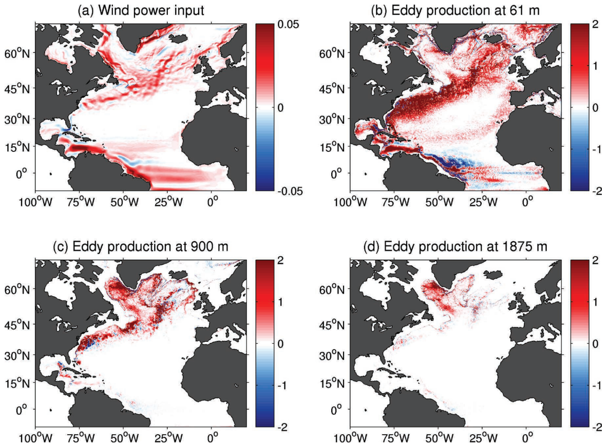
Fig. 4. (a) The wind power input to the North Atlantic Ocean ( \text{W m}^{-2} ). (b), (c), and (d) show the rate of APE released by baroclinic instability ( -\overline{\rho'w'^z}g; \times 10^{-5} \text{W m}^{-3} ) at 61 m, 900 m, and 1875 m, respectively. The color scale is saturated in order to reveal regions of moderate eddy activity. (Adapted from Zhai and Marshall 2013.)
