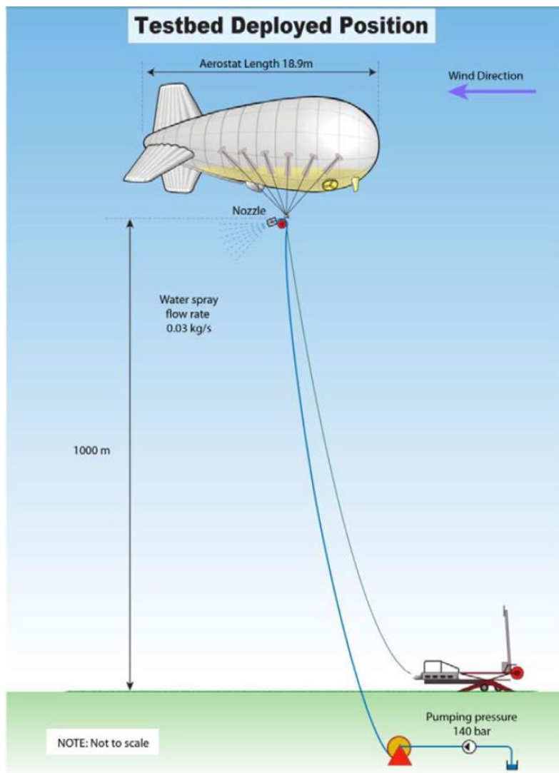
Figure 1 Schematic of the SPICE test bed proposal. Figure courtesy of Kirsty Kao, Cambridge University Engineering Department.
