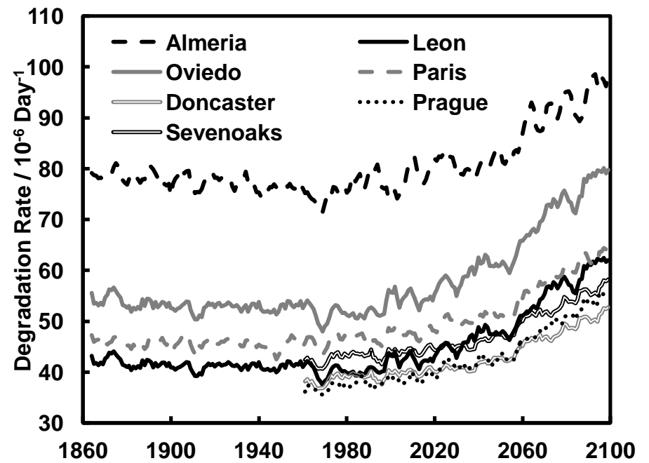
Figure C2: The projected relative degradation rate of paper using the TWPI damage function, from 1860 through to 2100 across the seven locations. The rate is shown as a 5 year smoothed average.
