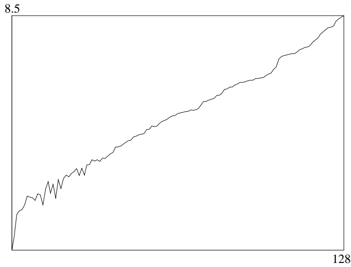
Figure 5: Graph of \log \log \Gamma_{n_j}(f_{33}) against j for n \leq 50,000 ; E_{f_{33}} = 18.984, W_{f_{33}} = 17.187, C_{f_{33}} = 17.869 .
