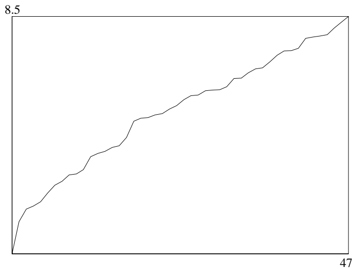
Figure 6: Graph of \log \log \Gamma_{n_j}(x^3 - x - 1) against j for n \leq 20,000 ; E_f = 6.807, W_f = 6.334, C_f = 6.398 .
