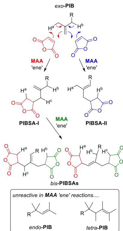
Scheme 2. Full Product Distribution of Species Formed in Industrial PIBSA Production (R = Polymer Chain)
