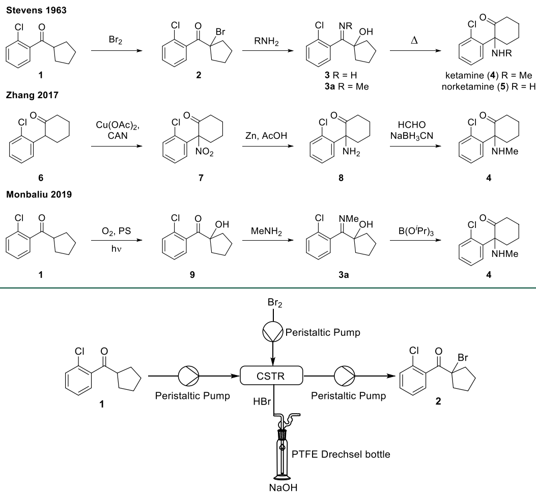
Figure 1. Bromination of 1 with Br 2 in a CSTR to form the \alpha -bromoketone 2. 4 mm OD PTFE tubing was connected via PTFE GL14 screw threads to a round-bottom flask (which served as the reactor) with GL14/B19 quick-fit adaptors.
