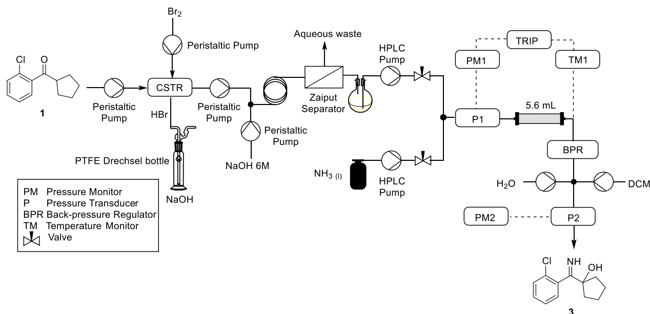
Figure 3. Reactor scheme for the daisy-chained synthesis of \alpha -hydroxy imine 3 from the ketone 1. The process involved bromination of 1 to form 2, in-line continuous-flow separation with a liquid–liquid membrane separator, high-pressure amination of the bromide 2 with liquid ammonia, and concomitant rearrangement to form the \alpha -hydroxy imine 3. Under these conditions, we were able to achieve 90% conversion to the imine 3 over two steps, as determined by 1 H NMR analysis. Moreover, when the same conditions were repeated without the inclusion of an internal standard, the imine 3 was isolated by precipitation from heptane in 82% yield.
