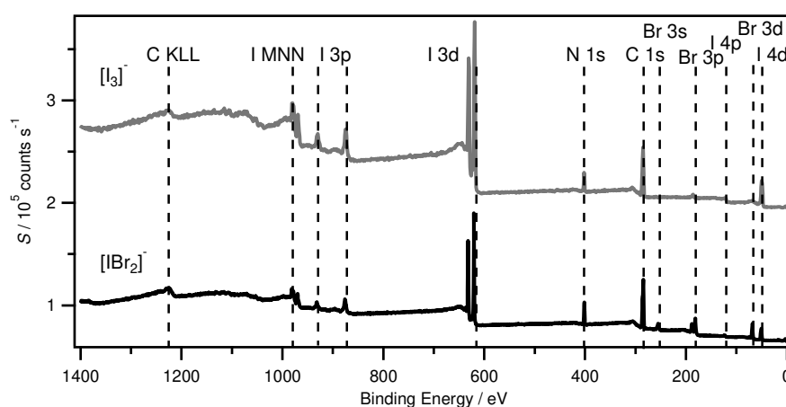
Figure 1 Survey XPS spectra for [\text{C}_8\text{C}_1\text{Im}][\text{I}_3] and [\text{C}_8\text{C}_1\text{Im}][\text{IBr}_2] .
