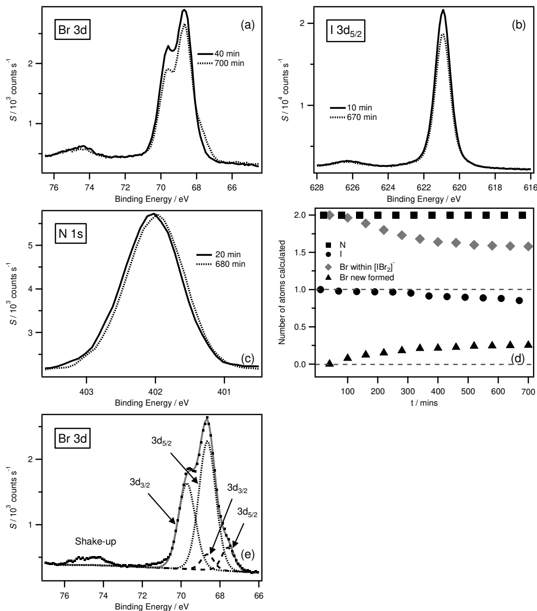
Figure 3 XPS spectra of [\text{C}_8\text{C}_1\text{Im}][\text{IBr}_2] (the first acquisition and the last acquisition) for: (a) Br 3d, (b) I 3d 5/2 and (c) N 1s. (d) Number of atoms for N, I, Br within [\text{IBr}_2]^- and Br (new formed) from XPS as a function of X-ray exposure time (STDEV available in Table S2). (e) Br 3d XPS spectrum with fittings for [\text{C}_8\text{C}_1\text{Im}][\text{IBr}_2] after 700 min of X-ray irradiation.
