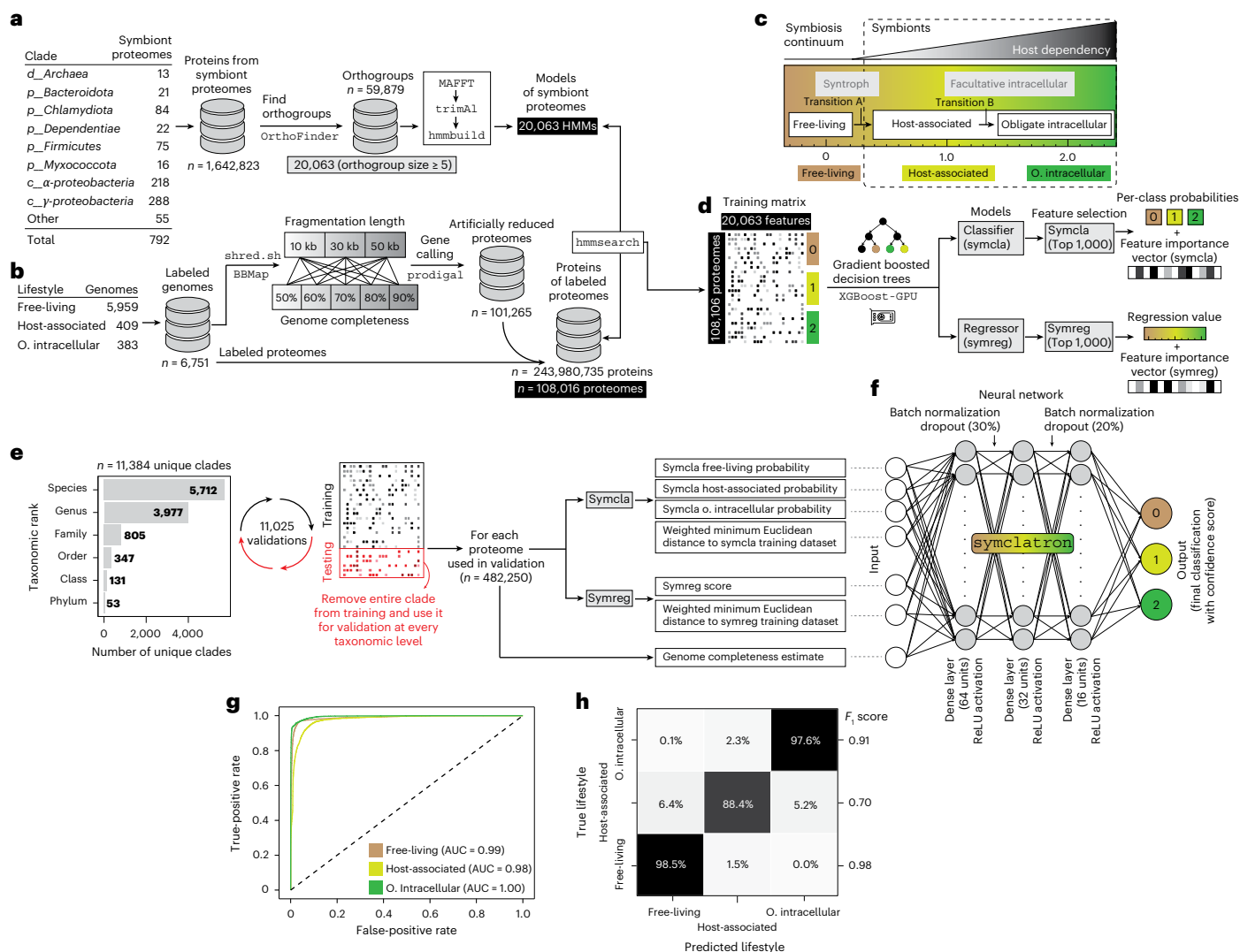
Fig. 1 | Developing an AI/ML framework for symbiotic lifestyle prediction in microbial genomes. a , Feature engineering workflow for detecting the genomic features specific to symbiotic genomes. b , Construction of a genus-level representative database of lifestyle-labeled genomes accounting for artificial genome reductions. c , Schematic of the symbiosis continuum concept applied in the labeling strategy for model training. d , Construction of the training matrix for the symbiont classifier (symcla) and symbiont regressor (symreg) using XGBoost. The final models were optimized for the most relevant 1,000 features. e , Strategy implemented to calibrate the final lifestyle prediction by training a neural network on the outputs of the out-of-fold validations. Right, the neural network was trained on 11,025 rounds of benchmarking and validations of the classifier and regressor models by blinding the models to entire clades from the
