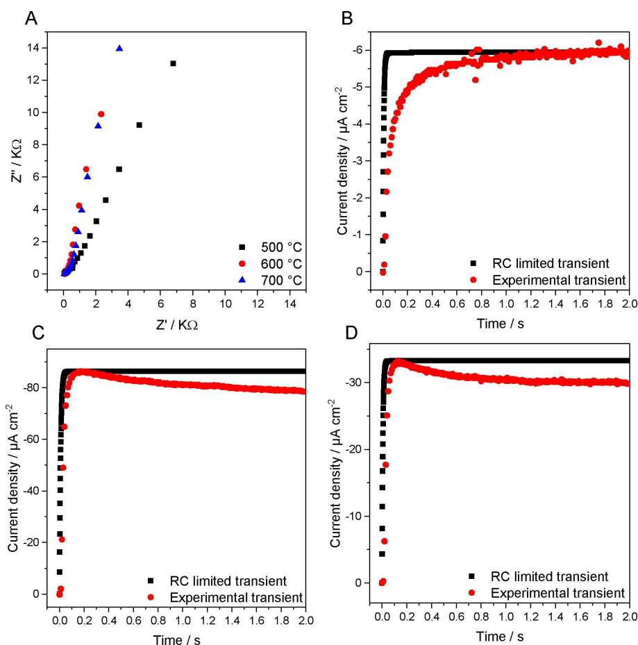
Figure 6. A) EIS measurements used for RC calculations in 0.1 M NaSO_4 with a DC of +0.61\ V_{RHE} and AC potential frequency range 10^5 –0.1 Hz with an amplitude of 5 mV under dark conditions. Experimental transient photocurrent plots from chronoamperometry measurements at +0.61\ V_{RHE} under chopped solar illumination with calculated RC limited transients for B) PFO_500 °C, C) PFO_600 °C and D) PFO_700 °C.
