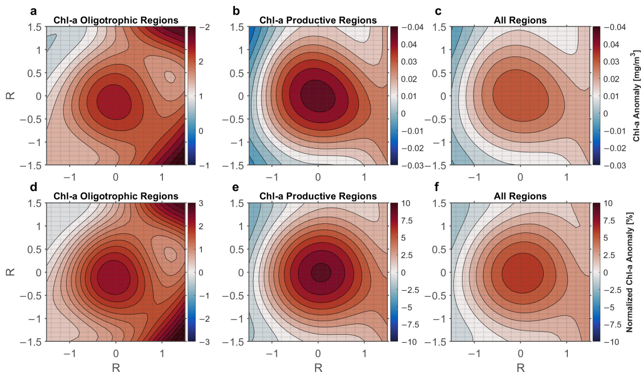
Figure 11. Composite surface Chl-a anomalies associated with fine-scale eddies. Absolute Chl-a anomaly composites for (a) Chl-a oligotrophic regions (monthly climatological Chl-a < 0.1 \text{ mg/m}^3 ), (b) Chl-a productive regions, and (c) all regions. (d–f) Same as (a–c), but for the corresponding composites normalized by the local monthly climatological Chl-a. Data are from the 20^{\circ} – 60^{\circ} latitude band over the study period (October 2023–September 2025).
