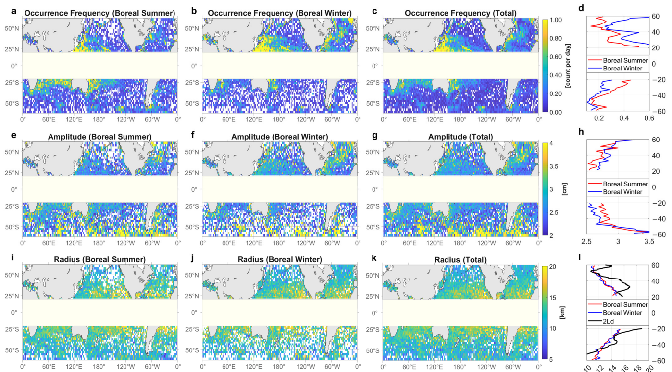
Figure 6. Seasonal characteristics of fine-scale eddies. Geographical distribution of fine-scale eddy occurrence frequency for (a) boreal summer, (b) boreal winter and (c) total eddies within a 2^\circ \times 2^\circ grid. (d) Zonal-mean eddy occurrence frequency over the study period (October 2023–September 2025). White areas in (a–c) denote regions without eddy detections. Red and blue lines in (d) denote boreal summer and boreal winter, respectively. (e–l) are the same as (a–d) but for eddy amplitude and equivalent radius, respectively. The black line in panel (l) indicates twice the mixed-layer instability scale.
