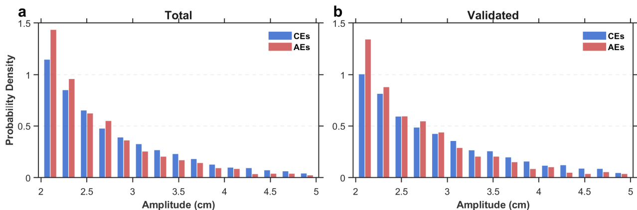
Figure 4. Polarity asymmetry in eddy amplitude during the “1-day fast-sampling” phase. PDFs of amplitude for (a) all detected eddies and (b) only temporally validated eddies. Blue and red bars denote CEs and AEs, respectively. Data are from the \pm 20 – 60^\circ latitude band during April–June 2023.
