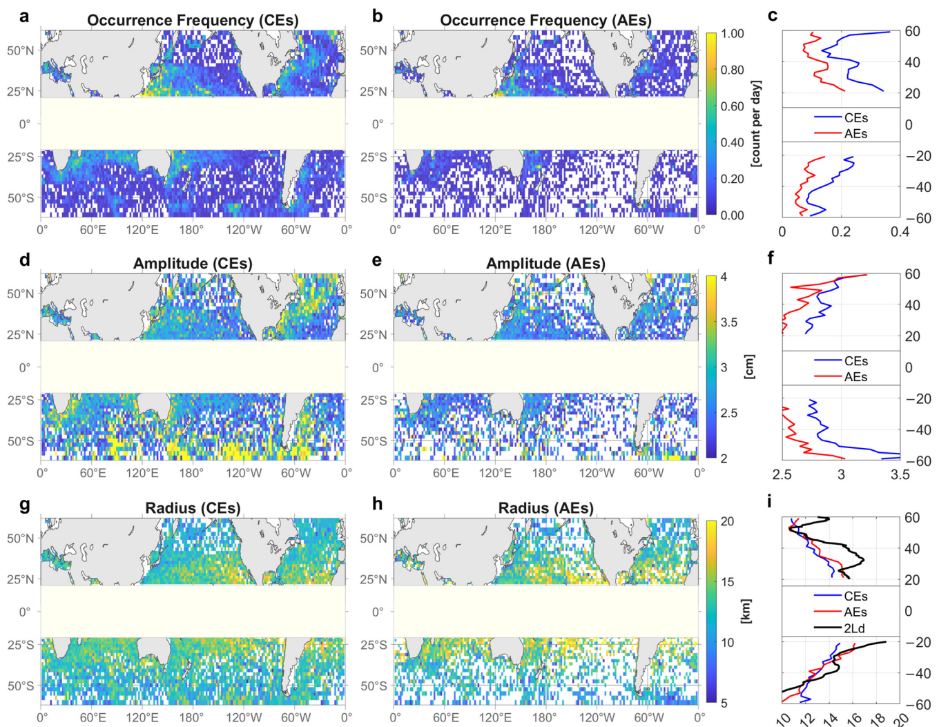
Figure 8. Polarity asymmetry of fine-scale eddies. Geographical distribution of fine-scale eddy occurrence frequency for (a) CEs and (b) AEs within a 2^\circ \times 2^\circ grid. (c) Zonal-mean eddy occurrence frequency over the study period (October 2023–September 2025). White areas in (a,b) indicate regions with no eddy detections. Blue and red lines in (c) denote CEs and AEs, respectively. (d–f) and (g–i) are the same as (a–c) but for eddy amplitude and equivalent radius, respectively. The black line in panel (i) indicates twice the mixed-layer instability scale.
