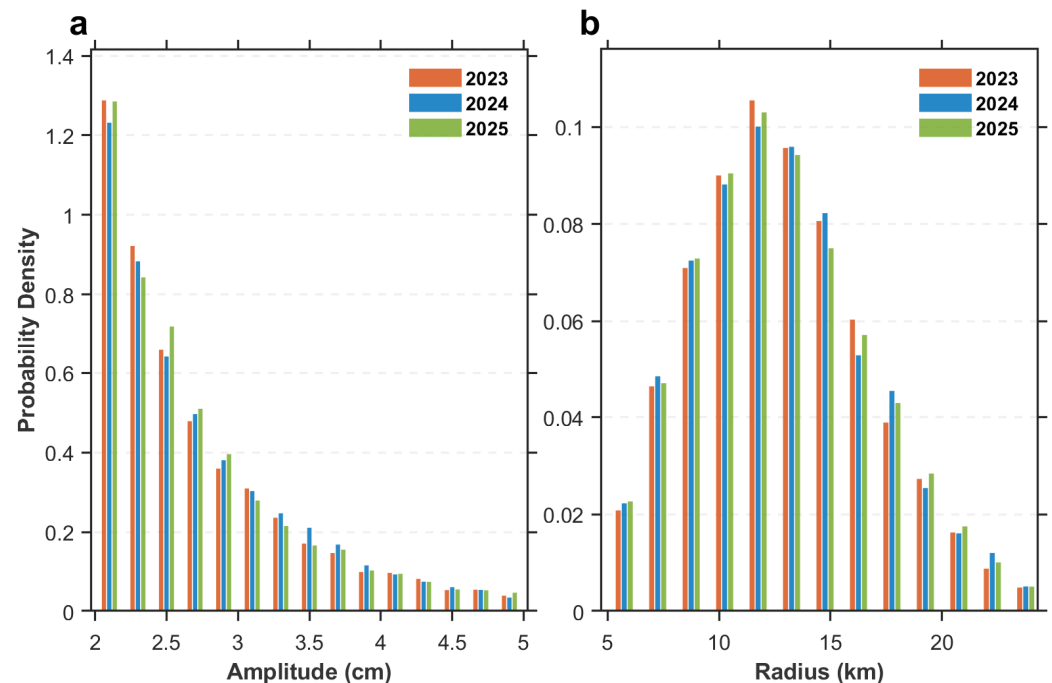
Figure 3. Comparison of eddy amplitude and radius distributions across different sampling phases. PDFs of (a) eddy amplitude and (b) equivalent radius for eddies detected during April–June in 2023 (“1-day fast-sampling” phase), 2024, and 2025 (21-day science phases).
