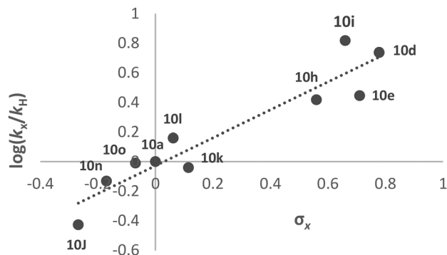
Fig. 3 Plot of \log(k_x/k_H) vs. Hammett substituent constant ( \sigma_x ) for glutathione addition to 4-( \alpha -arylvinyl)pyridines 10 ( \rho = 0.94 , R^2 = 0.89 ).
