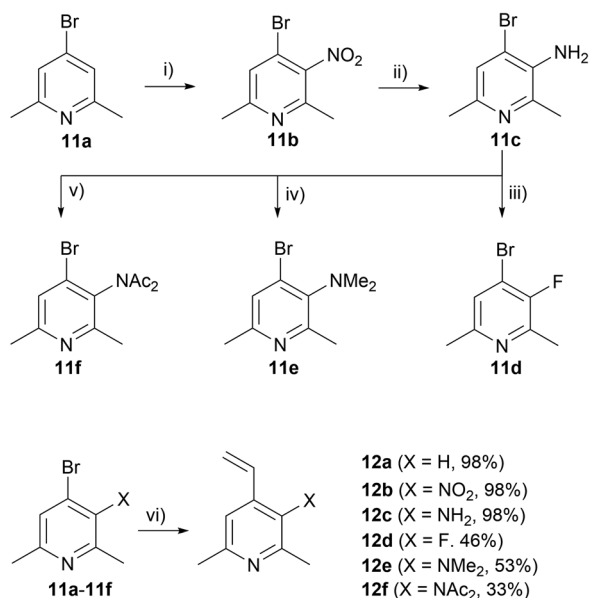
Scheme 5 Synthesis of 4-vinyl-2,6-dimethylpyridine 12a and 3-substituted derivatives 12b–f . (i) HNO 3 (3 eq.), H 2 SO 4 , 100 °C, 16 h. (40%). (ii) Fe (12 eq.), EtOH, HCl (aq) , Δ, 2 h. (99%). (iii) HBF 4 (2 eq.), NaNO 2 (1 eq.), H 2 O, 0 °C, PhMe, Δ, 16 h. (34%). (iv) 37% CH 2 O (2.5 eq.), HCO 2 H (6.5 eq.), Δ, 16 h (46%). (v) Ac 2 O (1.2 eq.), AcCl (2.6 eq.), NEt 3 (2.2 eq.), CH 2 Cl 2 , RT, 2 d. (59%). (vi) Potassium vinyltrifluoroborate (2 eq.), NEt 3 (3 eq.), PdCl 2 (dppf) (5 mol%), 2 : 1 PhMe/ i -PrOH, 90 °C.
