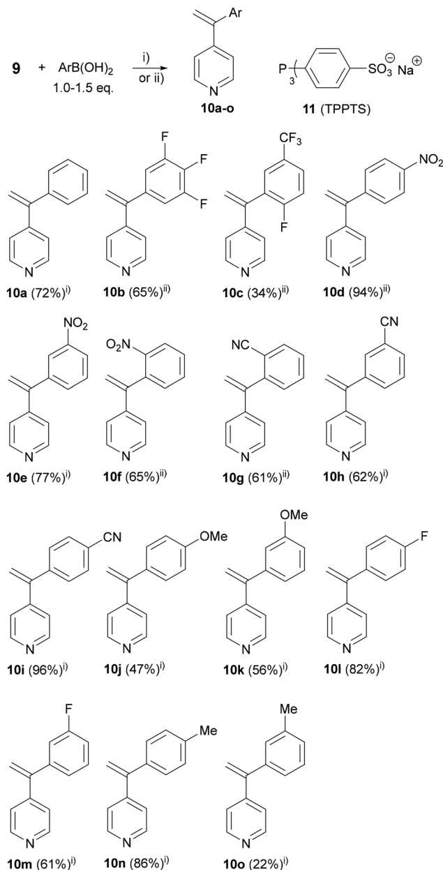
Scheme 3 Synthesis of 4-( \alpha -arylvinyl)pyridines 10a–10o. (i) \text{Pd}(\text{OAc})_2 (3–5 mol%), 11 (6–10 mol%), \text{K}_2\text{CO}_3 (3 eq.), 1:1 dioxane/ \text{H}_2\text{O} , 90^\circ\text{C} , 16 h. (ii) \text{Pd}(\text{PPh}_3)_4 (10 mol%), \text{K}_2\text{CO}_3 (3 eq.), 5:1 dioxane/ \text{H}_2\text{O} , 90^\circ\text{C} , 16 h.
