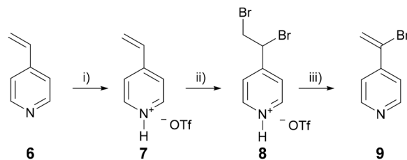
Scheme 2 Synthesis of 4-( \alpha -bromovinyl)pyridine 9. 17 (i) \text{TfOH} (1.1 eq.), \text{Et}_2\text{O} , 0^\circ\text{C} , 1 h. (quant.). (ii) \text{Br}_2 (2 eq.), \text{CHCl}_3 , 0^\circ\text{C} to RT, 2 h. (86%). (iii) \text{NEt}_3 (3 eq.), \text{MeCN} , 0^\circ\text{C} to RT, 3 h. (85%).
