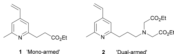
Fig. 1 4-Vinylpyridine based ADC linker groups 1 5,6 and 2 . 12
