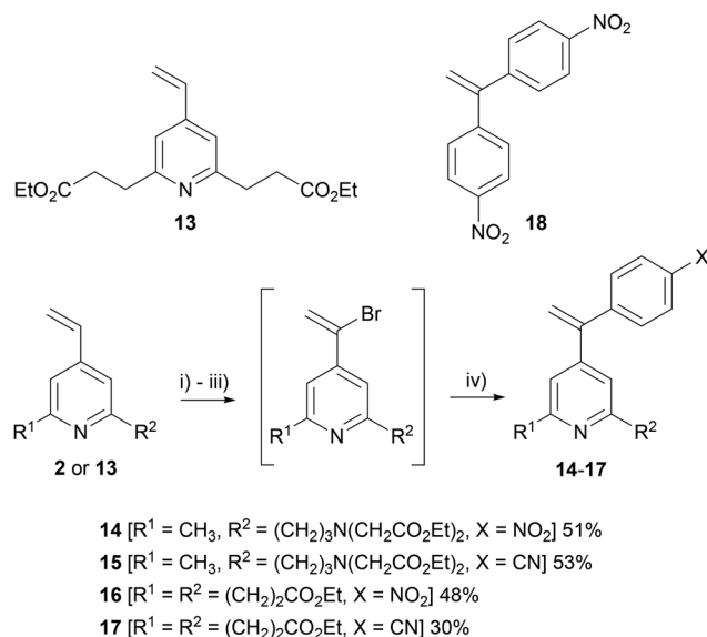
Scheme 6 Synthesis of activated functionalised ‘dual-armed’ 4-vinylpyridine derivatives 14–17 . (i) TfOH (1.1 eq.), CHCl 3 , 0 °C, 30 min. (ii) Br 2 (2 eq.), CHCl 3 , RT. (iii) NEt 3 (3 eq.), MeCN, RT. (iv) p -XC 6 H 4 B(OH) 2 (1.5 eq.), PdCl 2 (PPh 3 ) 2 (5 mol%), K 2 CO 3 (3 eq.), 5 : 1 dioxane/H 2 O, 90 °C.
