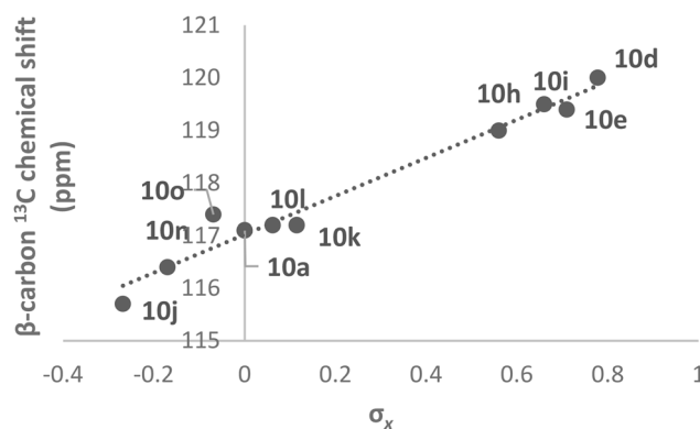
Fig. 4 Plot of \beta -carbon ^{13}\text{C} chemical shift vs. Hammett substituent constant ( \sigma_x ) 4-( \alpha -arylvinyl)pyridines 10 ( R^2 = 0.97 ).
