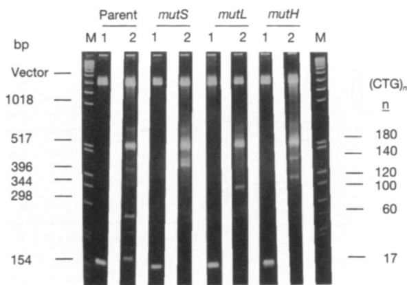
FIG. 2. Polyacrylamide gel electrophoretic analyses of Sac I– Hin dIII-digested DNAs containing CTG repeats grown in parent and mutator cell lines. Lanes 1, pRW3244 containing (CTG) 17 ; lanes 2, pRW3248 containing (CTG) 180 grown in the parent KA796 strain and in the mutator cell lines ( mutS , mutL , and mutH , respectively). Lanes M, 1-kb marker. The sizes of the restriction fragments along with their numbers of triplet repeats are shown.
