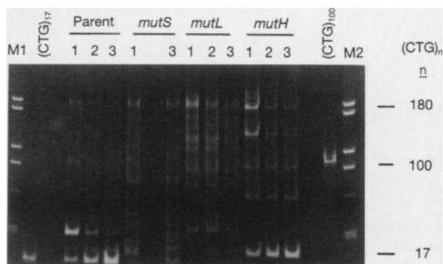
FIG. 4. Polyacrylamide gel analysis of Hind III– Sac I restriction fragments of pRW3247. Lanes 1, 2, and 3 show Hind III– Sac I restriction fragments of pRW3247 isolated from parent, mutS , mutL , and mutH strains grown for about 40, 60, and 80 generations, respectively. M1 is the 1-kb marker, and M2 is the marker of pBR322 digested with Msp I endonuclease. The lanes designated (CTG) 17 and (CTG) 100 are Hind III– Sac I digests of pRW3244 and pRW3246, respectively.
