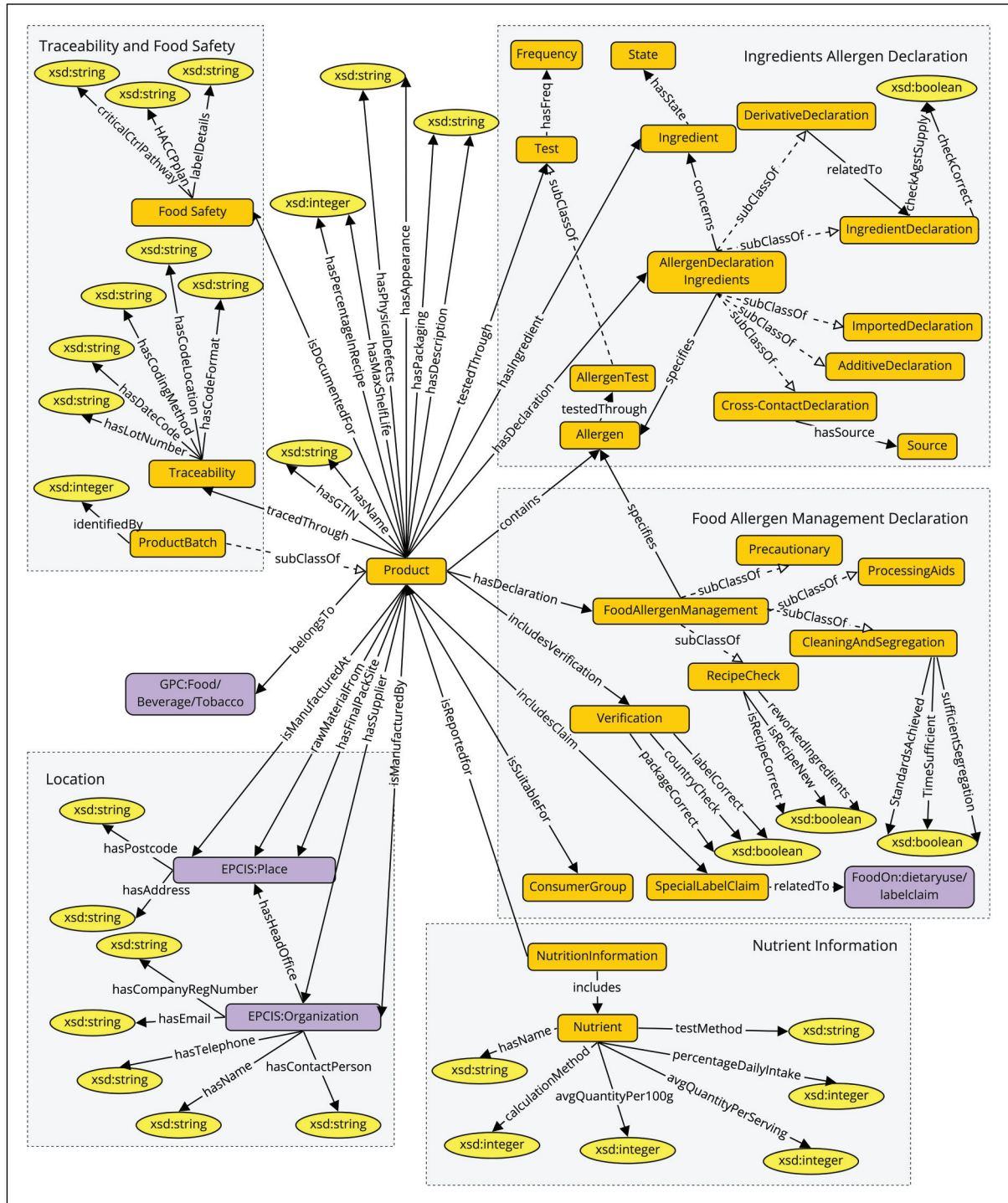
Figure 2. Schema diagram for Food Allergen Traceability Ontology (FATO), with classes from external sources shown in purple.
