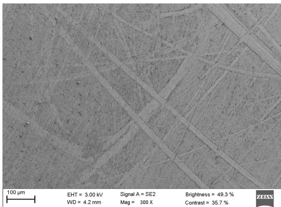
Fig. 42 Scanning electron microscope (SEM) image of mono- and few-layer graphene sheet consists of the nanostripes on Si/SiO 2 substrate with atomically flat surface achieved using pressure of \sim 200 Pa at rubbing (with bulk graphite powder) circular cycles of 500. The rubbings are performed manually. Figure adapted from [250]
